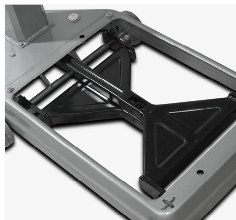
Double V-shape lever
